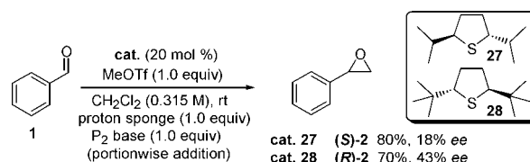
Scheme 4. Catalytic Asymmetric Methylene Transfer
