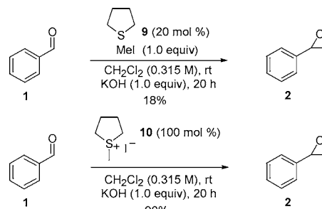
Scheme 2. Preliminary Experiments: Identification of Sulfonium Salt Formation as the Problematic Step
